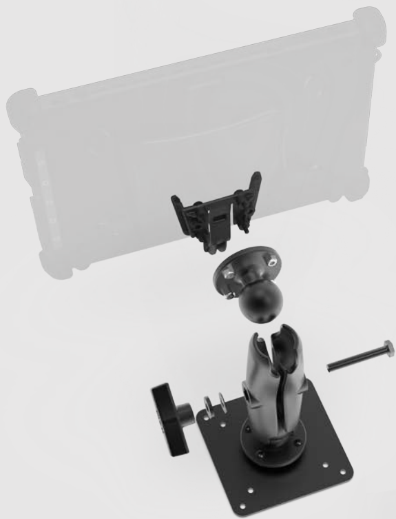
Fixed Mounting
